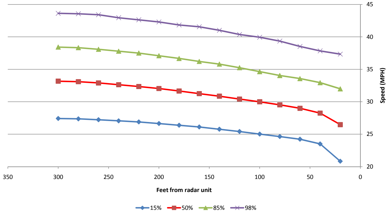
Selected Speed Percentiles of Vehicles Approaching the Radar
