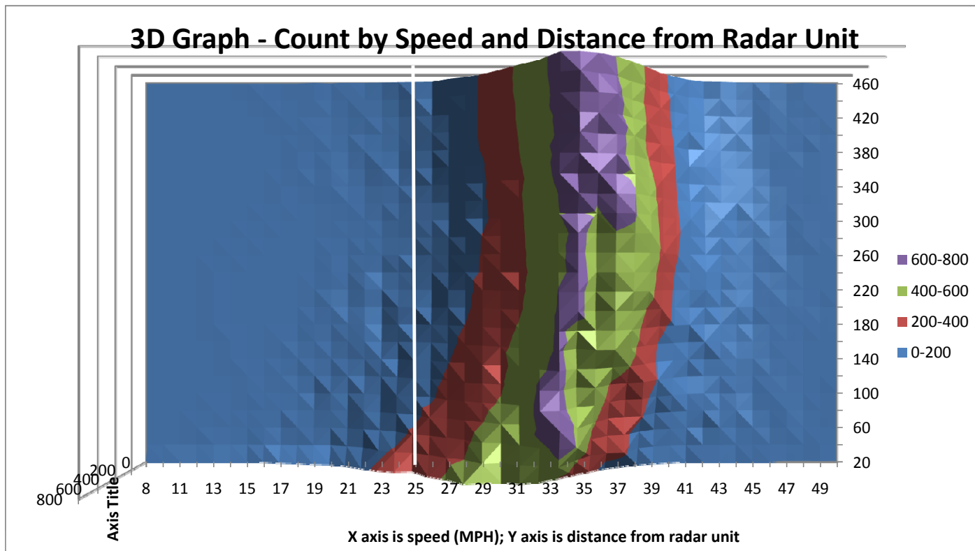
3D Graph - Count by Speed and Distance from Radar Unit
